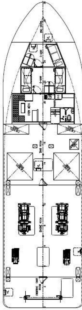
BOTTOM PLAN
