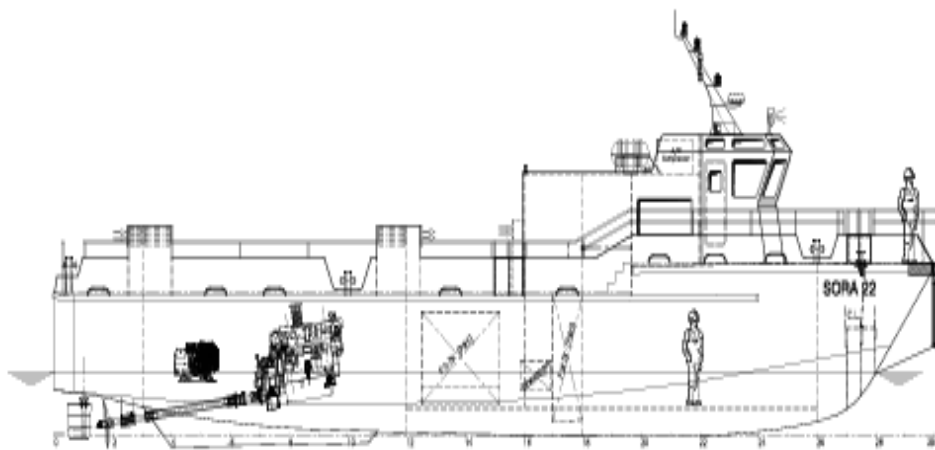
PROFILE
