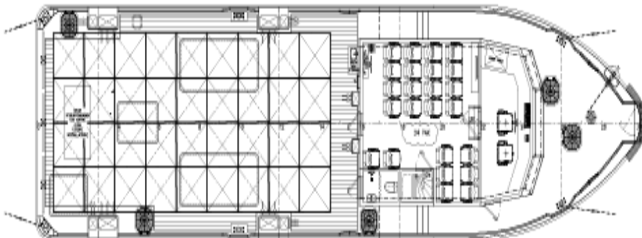
MAIN DECK PLAN
