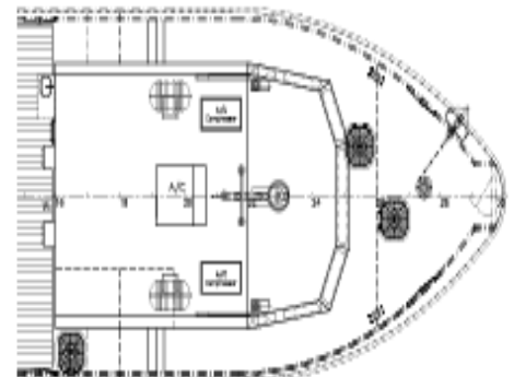
TOP OF DECKHOUSE
